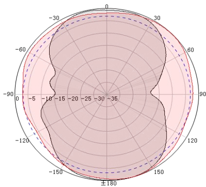
Figure 2 - E-Plane @ 2100MHz
