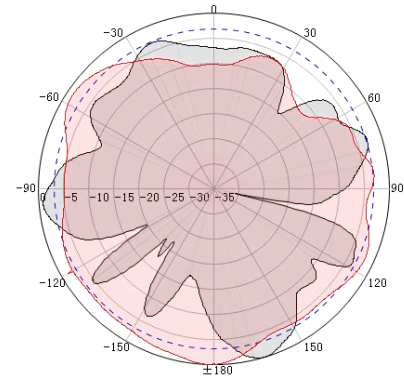
Figure 4 - E-Plane @ 920MHz
